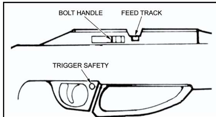
Figure 6-1-1 Safety Catch
